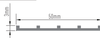
CHANNEL TREAD
