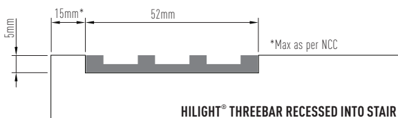
HILIGHT® THREEBAR RECESSED INTO STAIR
