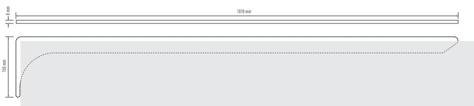
FIN - LARGE PRODUCT CODE: CPSBDF1010-150
